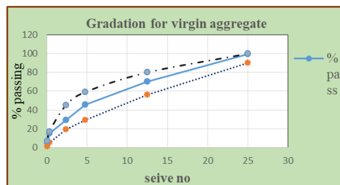
Figure 6 Blending curve for virgin aggregate with specification
