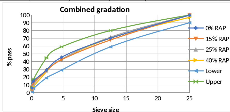
Figure 7 Final blending Curve for Combined Gradation of RAP Material and Fresh Aggregates
