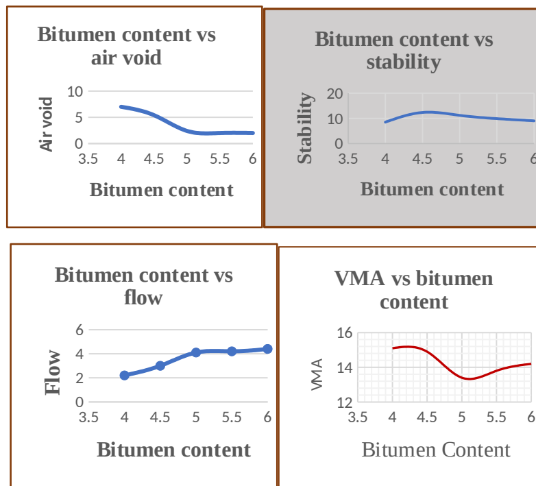
Figure 8 Marshall Property graph results for control mix 0% RAP
