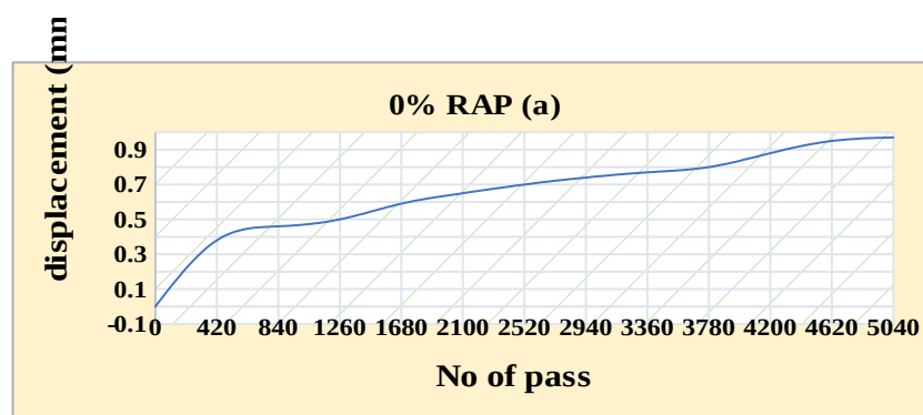
Figure 9 Wheel tracking test result for 0%
